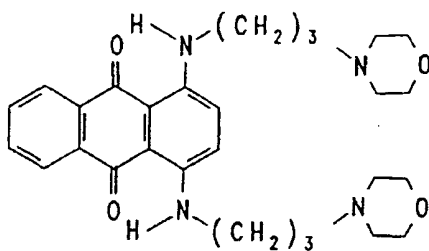
Compound 1c
